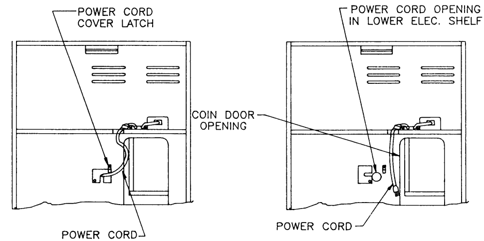
3-D VIEW OF POWER CORD ROUTING
