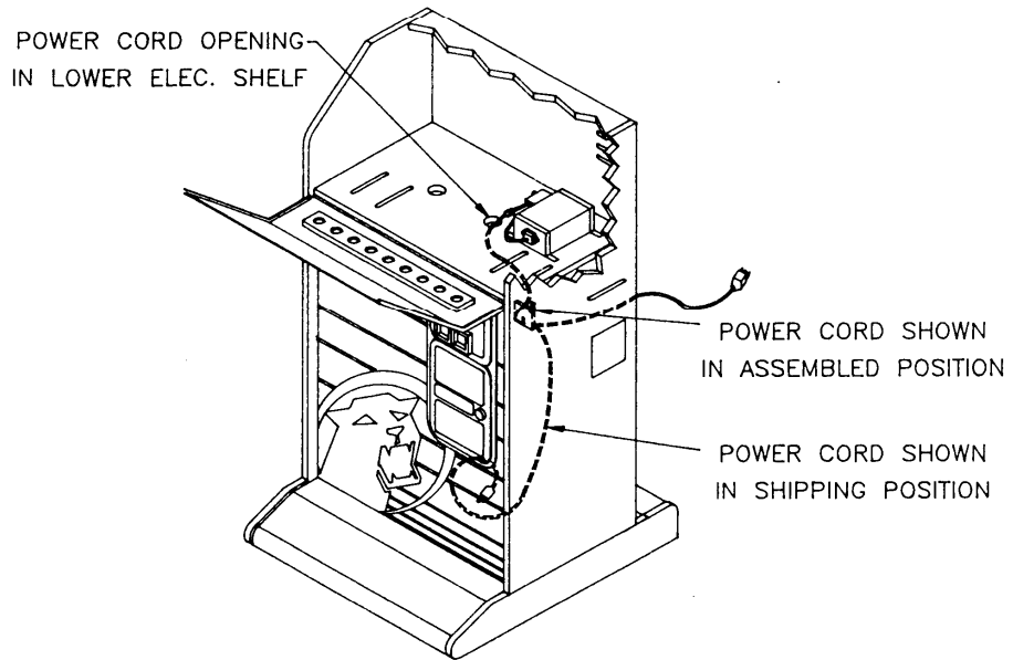
3-D VIEW OF POWER CORD ROUTING
