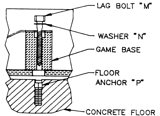
Figure 11. Fasten to a concrete and wood floor
