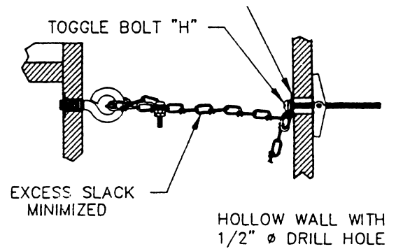
Figure 7. Close-up toggle bolt
