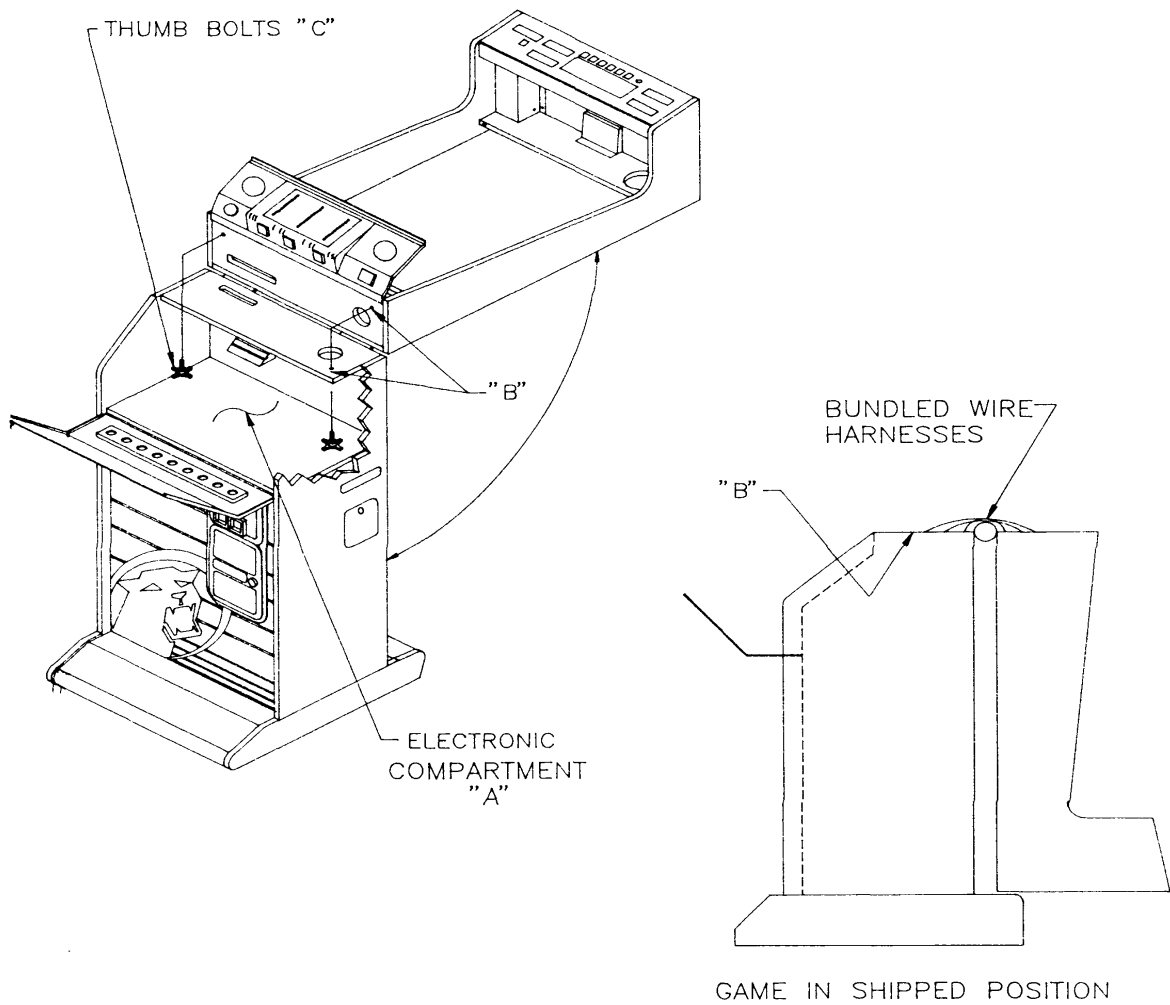
Figure 1. Game in shipped position
