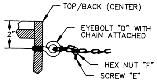
Figure 5. Eye bolt and chain fastened to game
