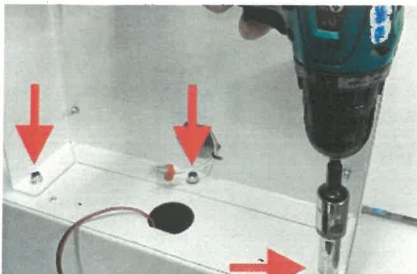
Install 3 nuts and washers
